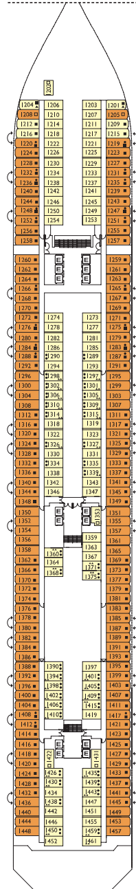
DECK 1 IRMA
